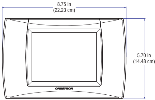
STX-1700C Touchpanel – Top View (face up)
